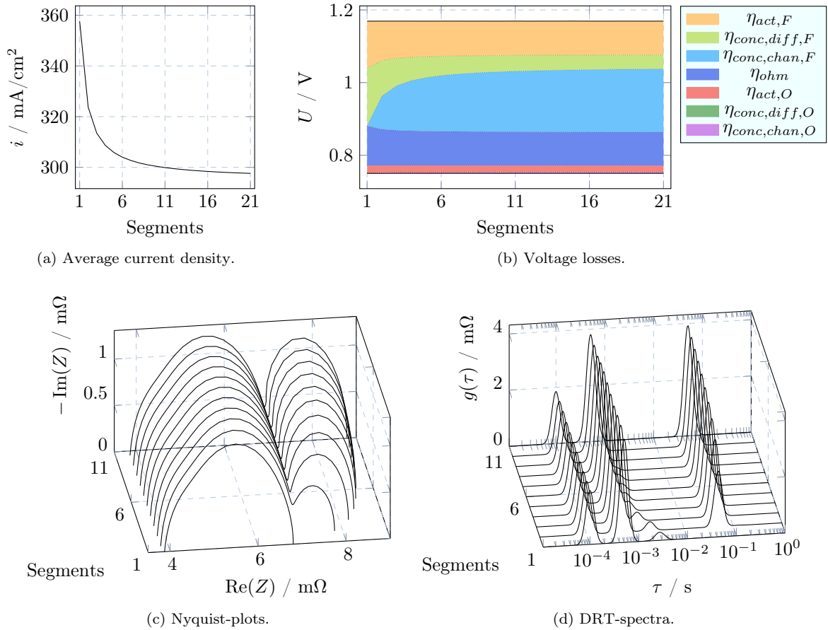
Figure 7: Impact of number of segments on the cell performance, when fueling it with dry hydrogen at 0.75 V.
