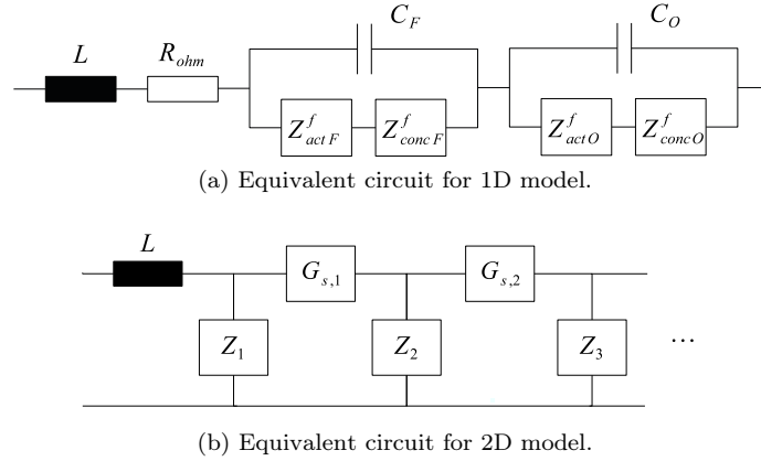
Figure 5: Equivalent circuit used.
